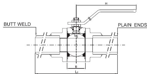
WELDED NIPPLES
