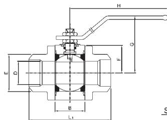
SCREWED NPT-BSPP
